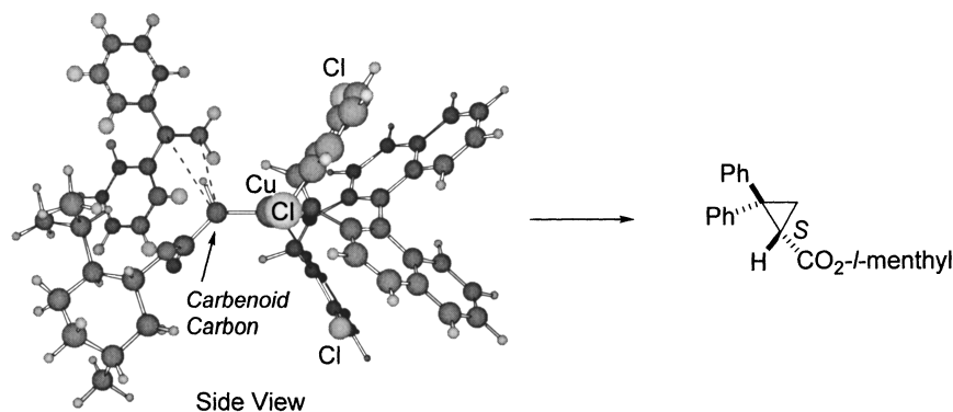
Fig. 2. Proposed approach of 1,1-diphenylethylene.
