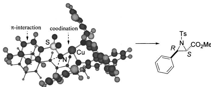
Fig. 4. Proposed approach of methyl cinnamate.
