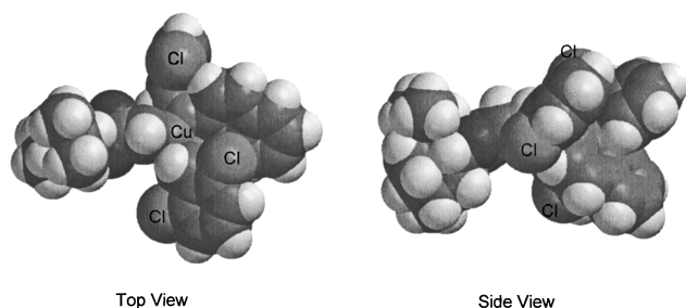
Fig. 1. Optimized structure of the Cu(I)-BINIM-DC complex calculated by PM3.
