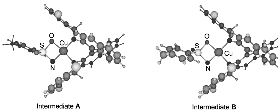
Fig. 3. Optimized structure of intermediates A and B.
